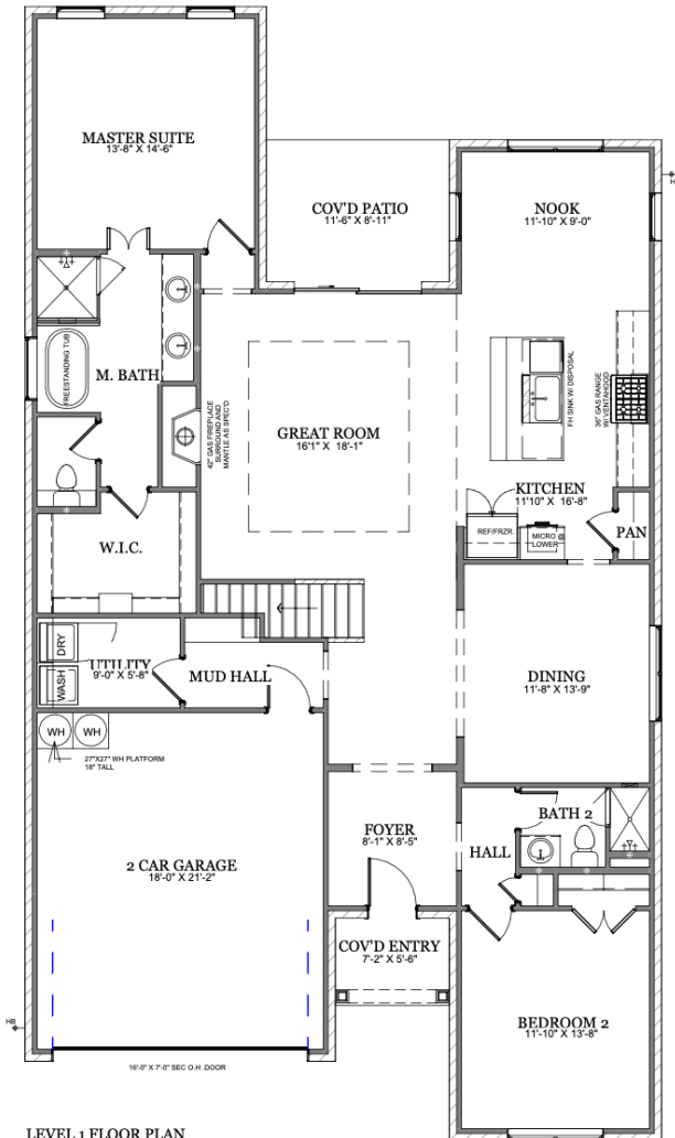
LEVEL 1 FLOOR PLAN
